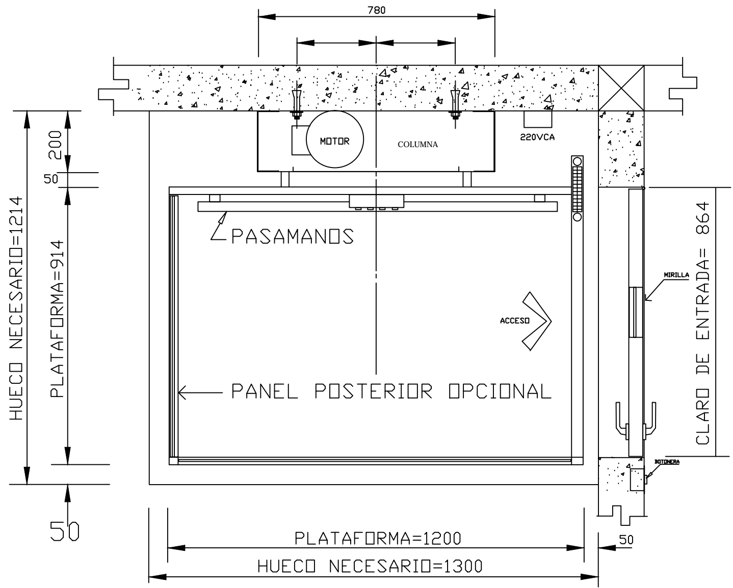
PLANTA MECANICA HPE-210 CABIN
